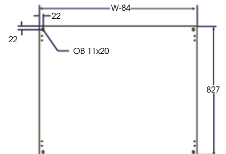
MOUNTING PLATE
