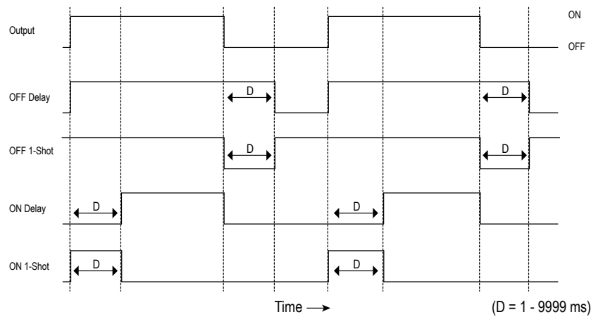
Figure 14. Delays/Timers
