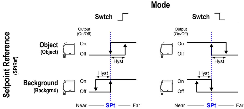
Figure 12. How hysteresis affects the two discrete output window modes
