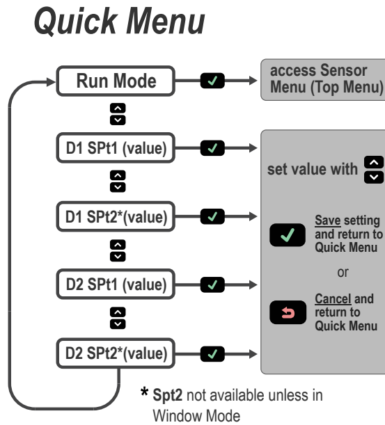
Figure 7. Quick Menu Map (Window Mode)
