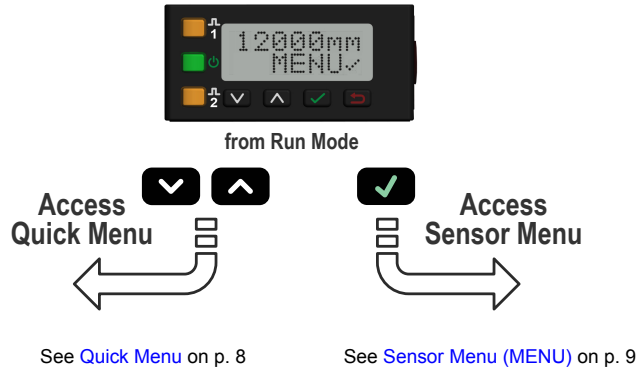
Figure 6. Accessing the Menus
