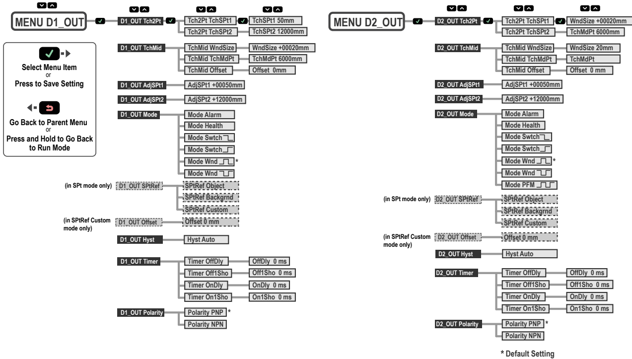
Figure 9. Discrete Output Menu Maps
