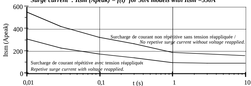
Fig.3 Surcharge de courant : I_{tsm} (A_{peak}) = f(t) pour modèle 50A( I_{tsm}=550A ) Surge current : I_{tsm} (A_{peak}) = f(t) for 50A models with I_{tsm} = 550A
