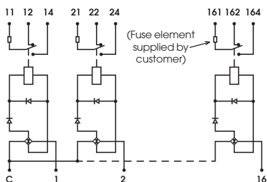
Wiring diagram of electromechanical relays with 24VDC non-polarised power supply (12VDC modules available on request)
