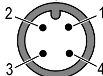
4-pin M12 male quick disconnect
