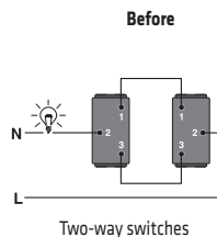
Control from two points (2 two-way switches)
