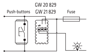
Control and adjustment from two points (1 dimmer + 1 NO push-button)
