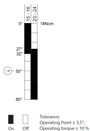
Operating diagram
