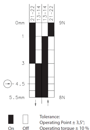
Operating diagram
