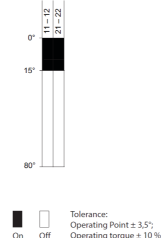
Operating diagram
